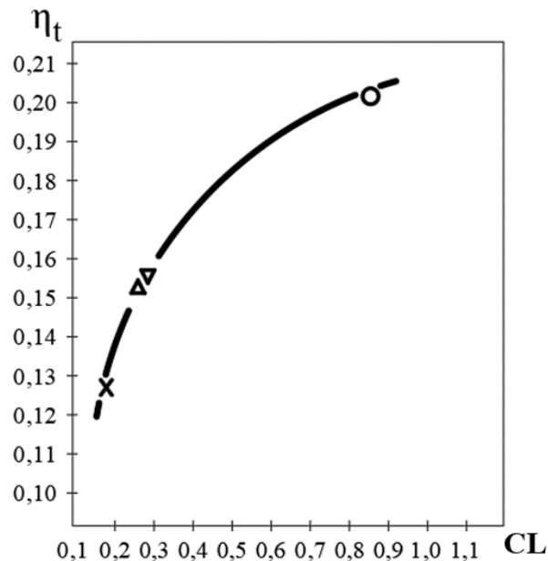
Fig. 2. Cycle efficiency in the function of CL criterion for various working fluids: x - acetone, o – methanol, Δ – benzene, ▽- toluene
