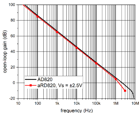
Fig. 11. Open-loop gain versus frequency for aRD820 at source voltage \pm 2.5 V and AD820
