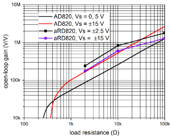
Fig. 9. Open-loop gain vs. Load Resistance at normal temperature for aRD820 at source voltage \pm 2.5 V and \pm 15 V, and for AD820 at source voltage 0, 5 V and \pm 15 V
