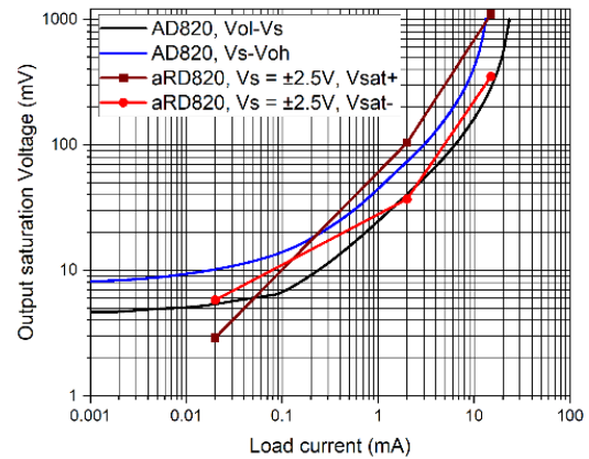
Fig. 10. Output saturation voltage for positive and negative rails V_s load current for aRD820 at source voltage \pm 2.5 V, and for AD820
